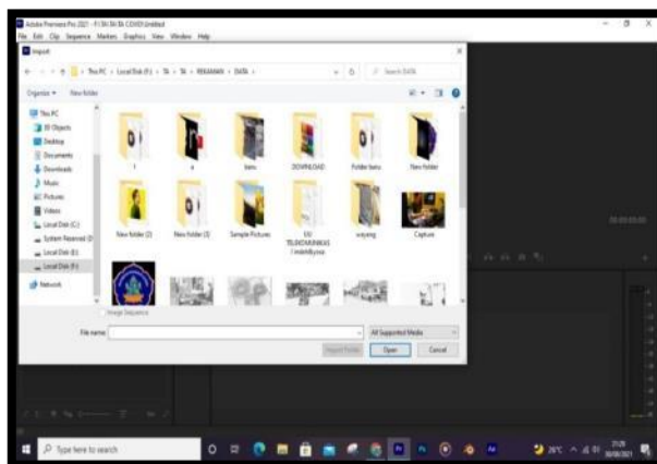
Gambar 4.2 Import Video
