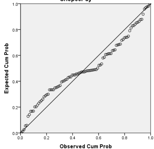
Normal P-P Plot of Regression Standardized Residual Dependent Variable: Keputusan Penggunaan Teknologi Keuangan (Fintech) ShopeePay
