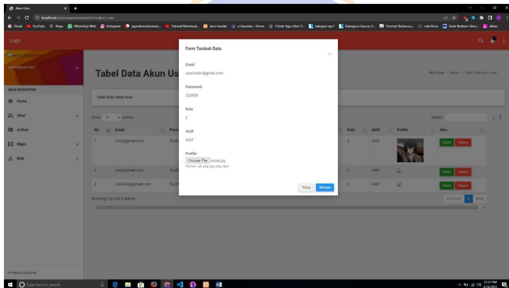
Gambar 6 Menambah User
