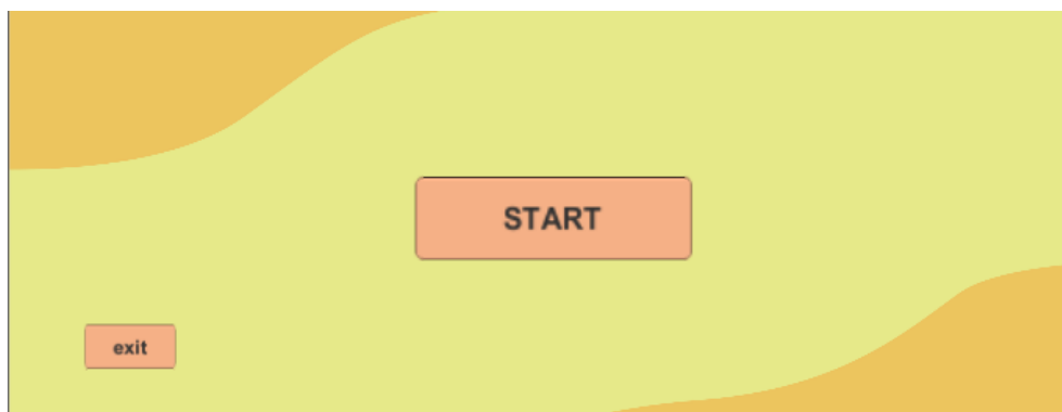
Gambar 1 Halaman Start
