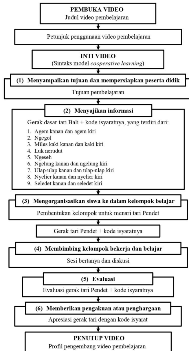
Gambar 5. Flowchart
