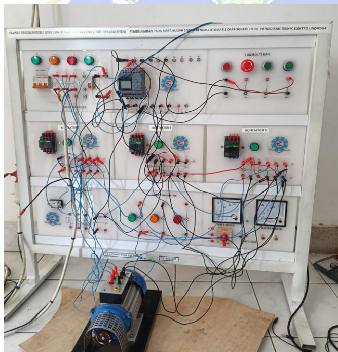
Gambar 2 : Uji Coba Trainer Programmable Logic Controller (PLC) Siemens Logo!
