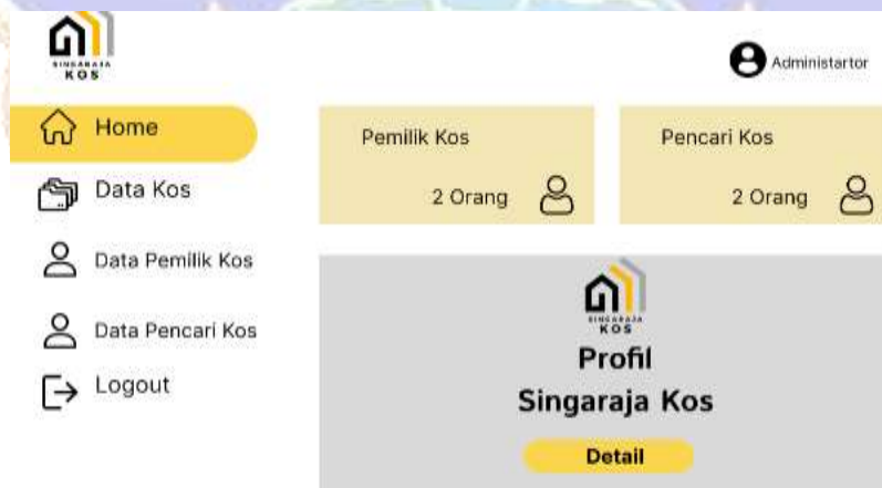
Gambar 20 Dashboard Admin
