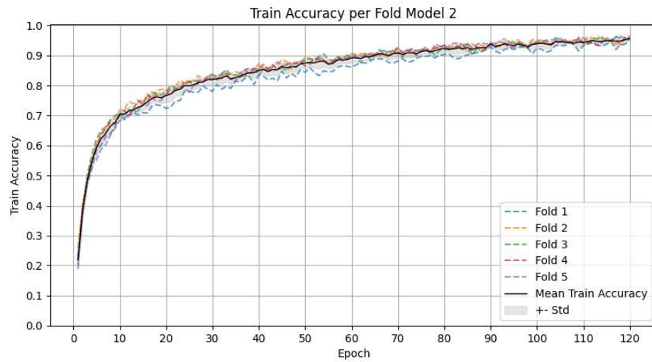
Lampiran 3 Performa Akurasi Model 2
