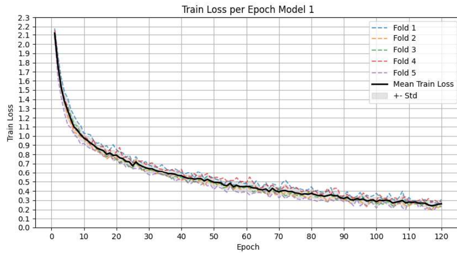
Lampiran 2 Performa Loss Model 1
