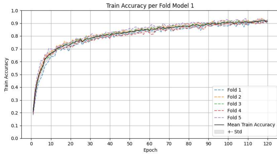
Lampiran 1 Performa Akurasi Model 1
