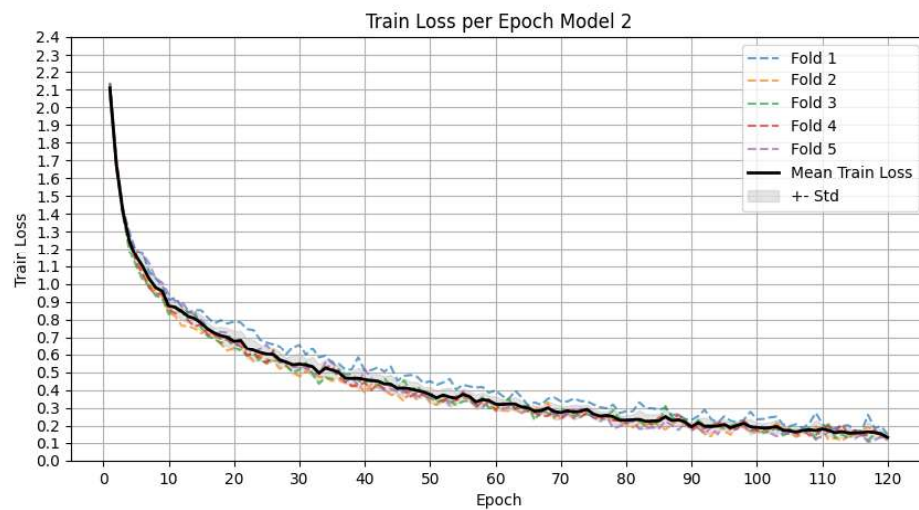
Lampiran 4 Performa Loss Model 2
