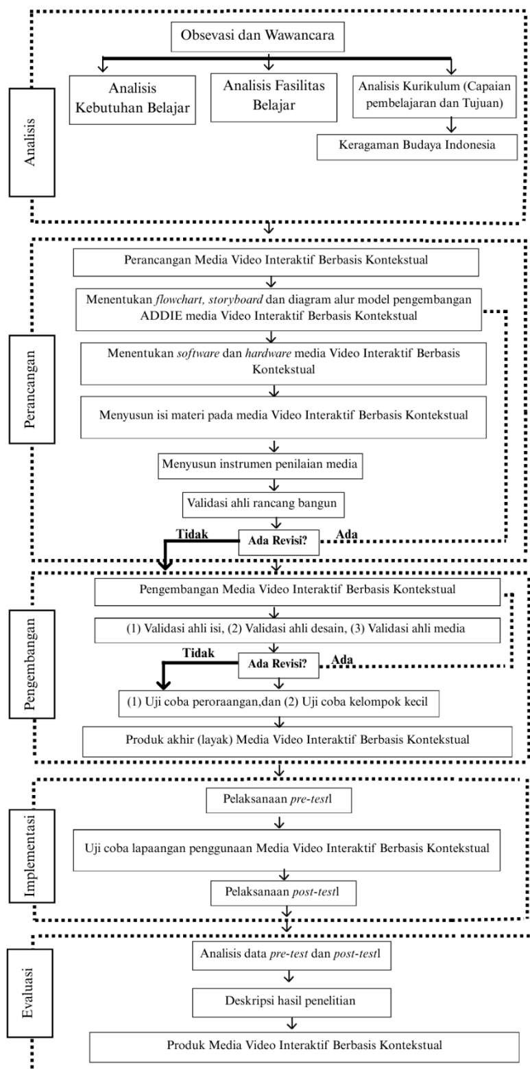
Lampiran 0. 9 Diagram Alir Video Interaktif Berbasis Kontekstual
