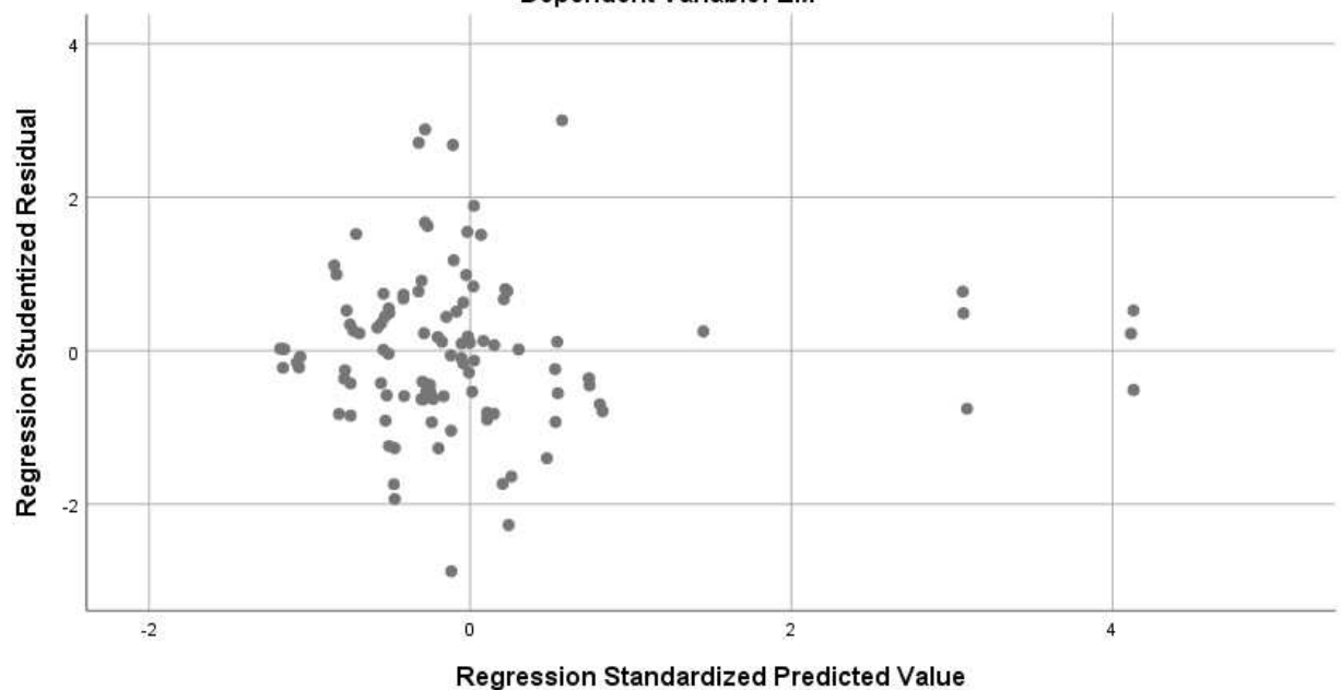
Scatterplot
