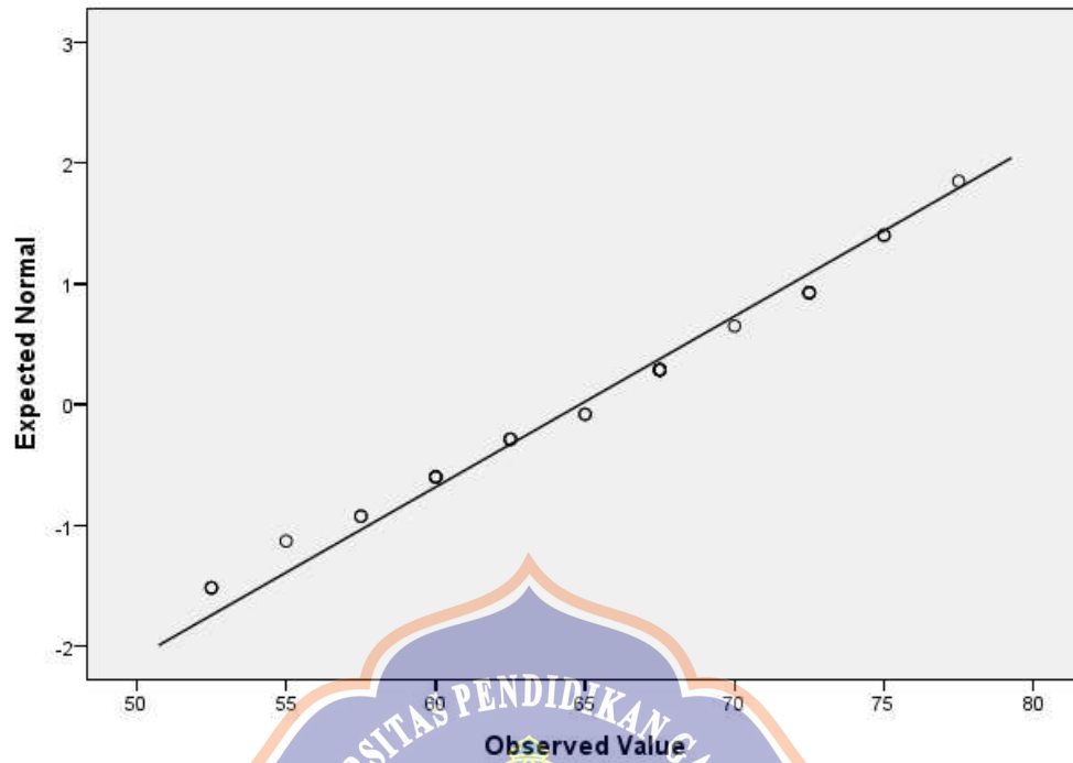
Normal Q-Q Plot of Hasil Belajar for K= Posttest Kontrol
