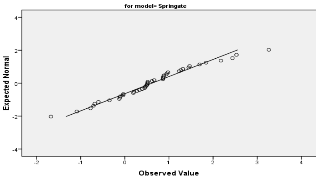
Normal Q-Q Plot of Score Prediksi
