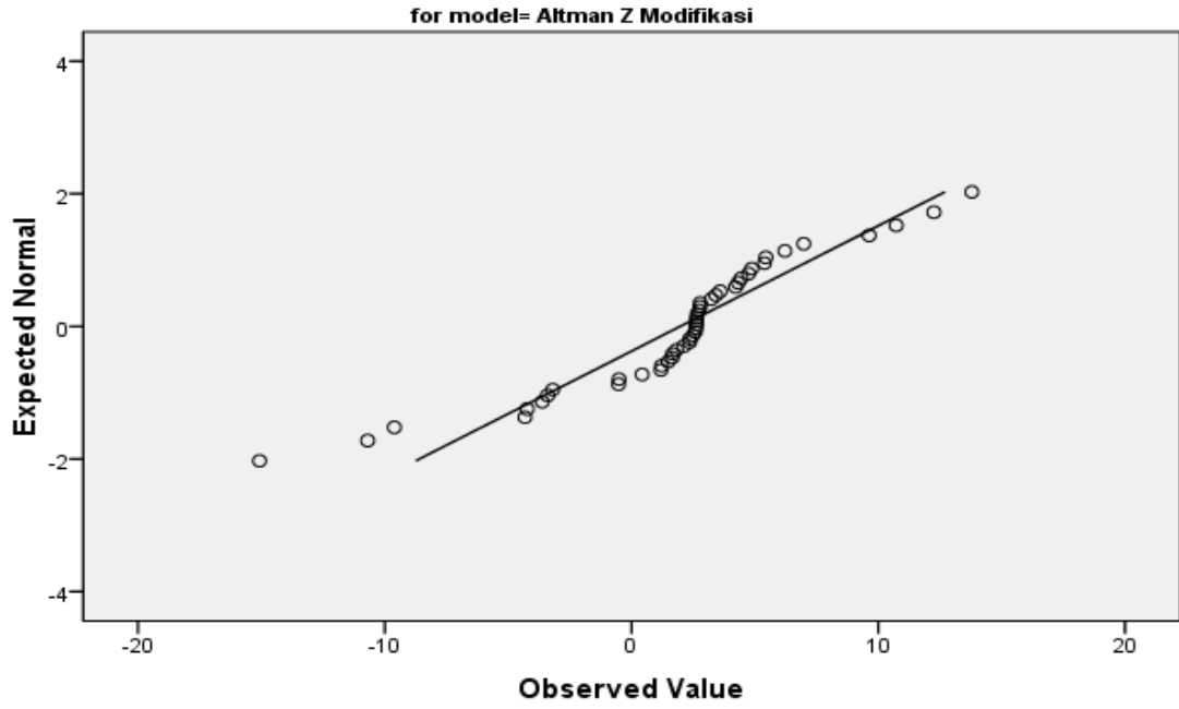
Normal Q-Q Plot of Score Prediksi
