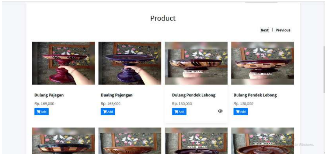
Gambar 4 Halaman User
