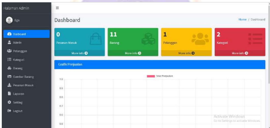
Gambar 2 Halaman Admin
