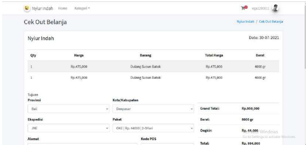
Gambar 34 Halaman Checkout
