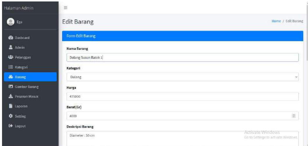
Gambar 22 Edit Barang
